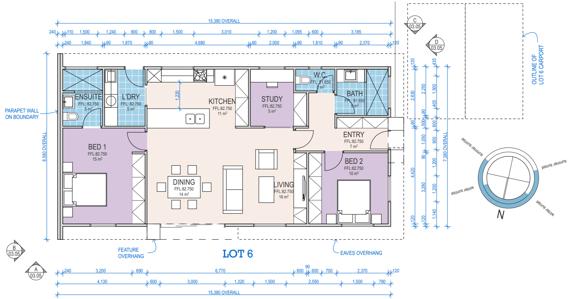
LOT 6 FLOOR PLAN 1:100
