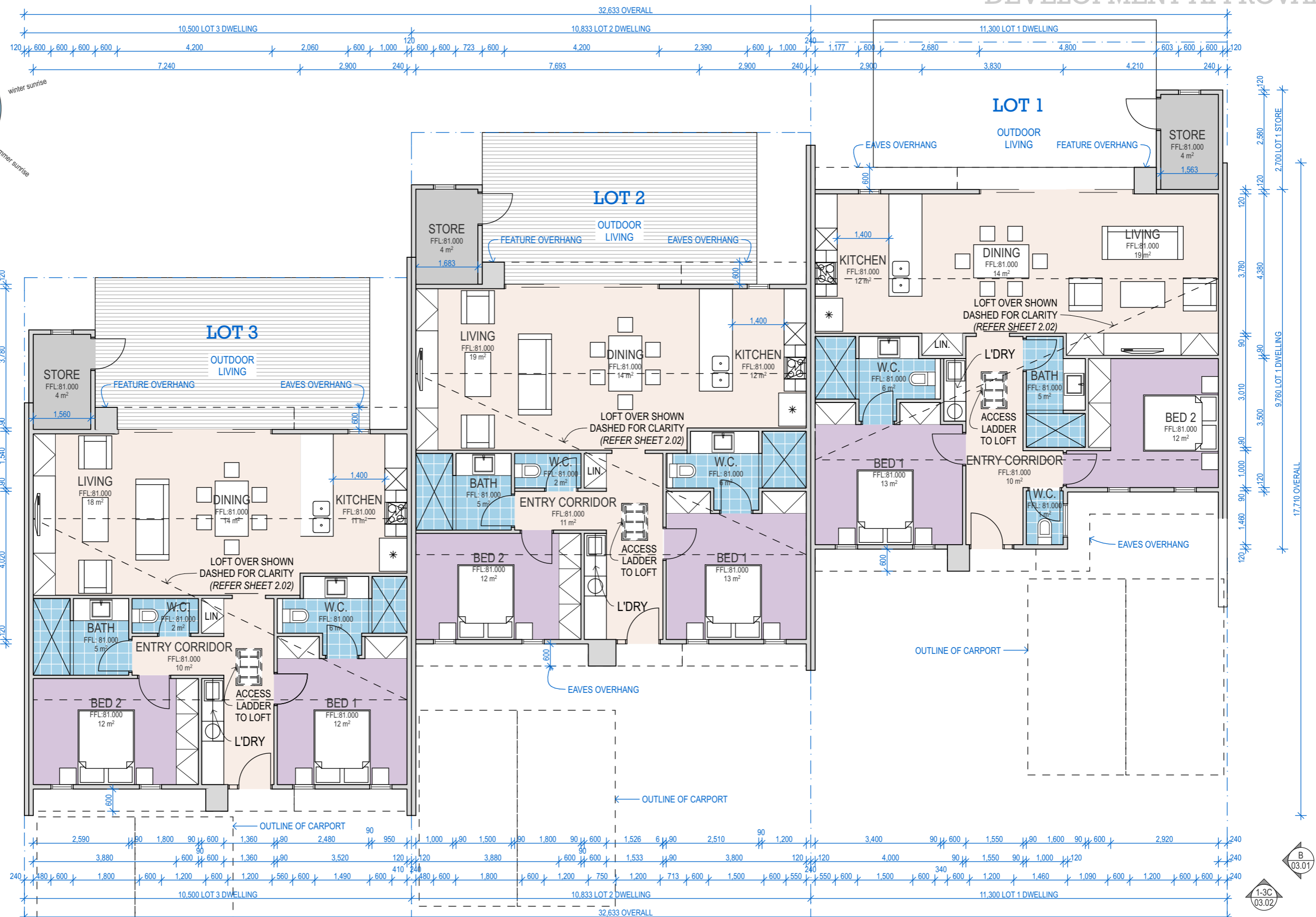
UNITS 1-3 FLOOR PLANS 1:100
